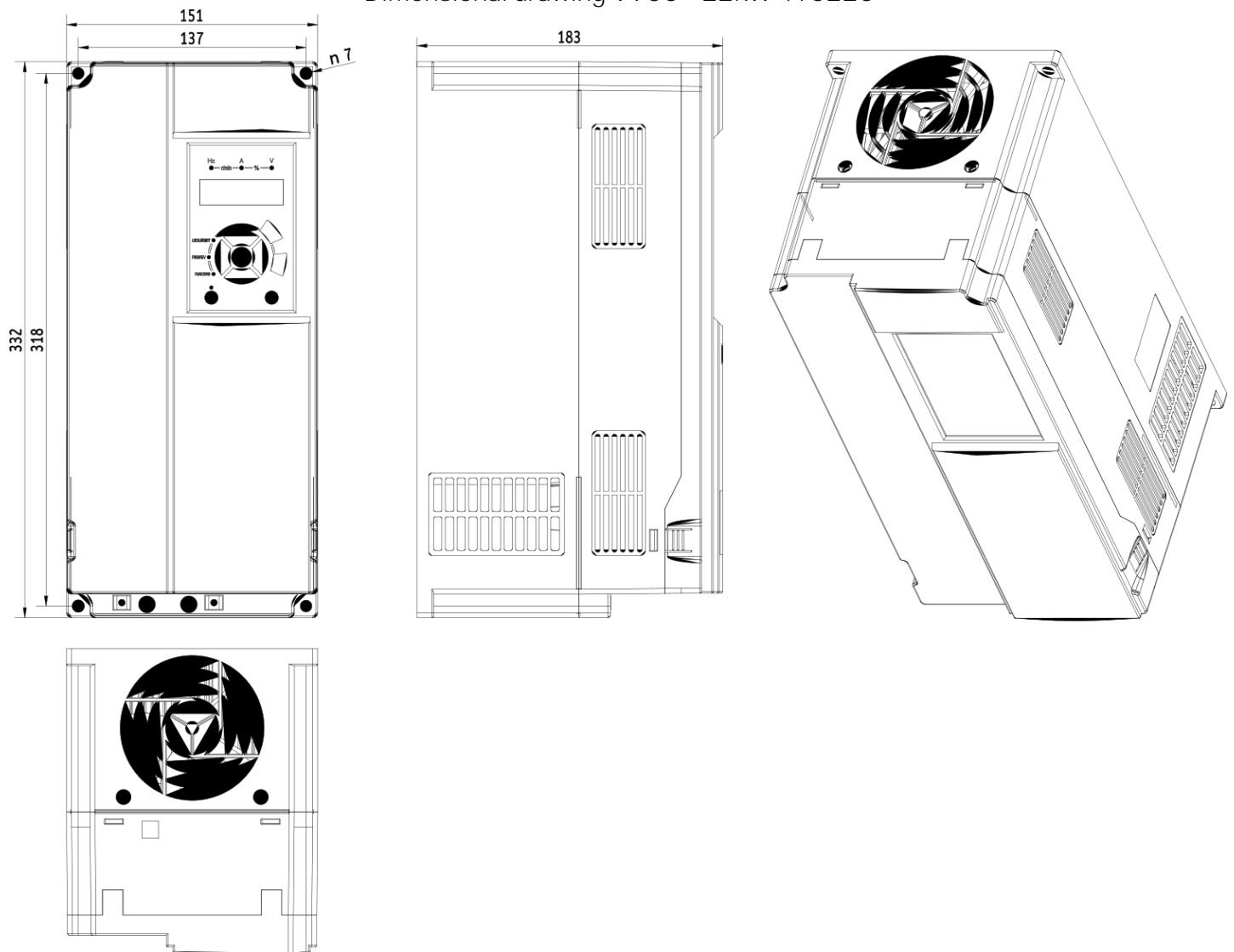
Dimensional drawing V900 - 22kW 4T0220
