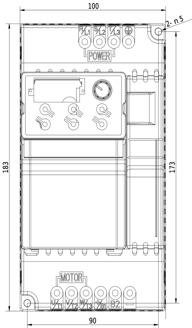
Dimensional drawing V800 - 4kW 4T0040
